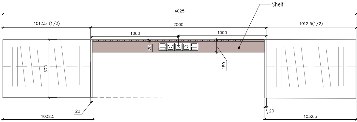
VIEW TOP
