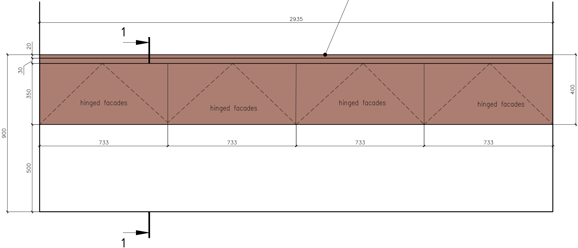
VIEW 1
