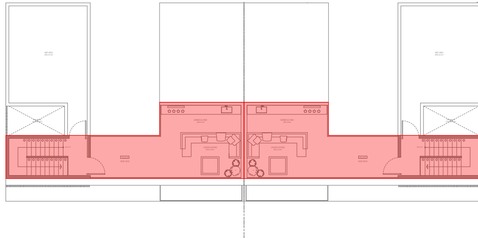
ROOF DECK PLAN
