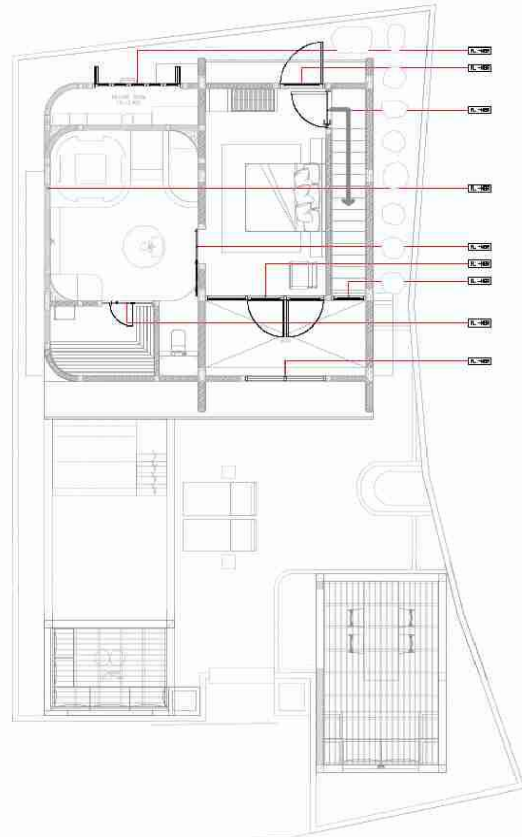
DOOR AND WINDOW PLAN VILLA A Scale 1 : 100
