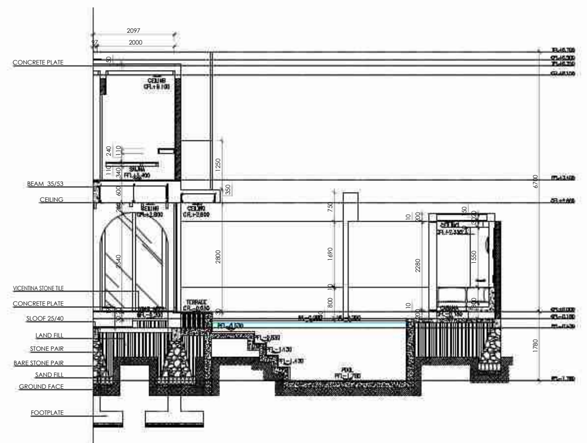
BLOW UP SECTION 2 VILLA C Scale 1 : 100
