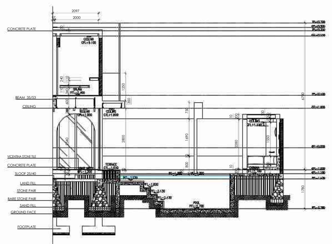
BLOW UP SECTION 2 VILLA B Scale 1 : 100
