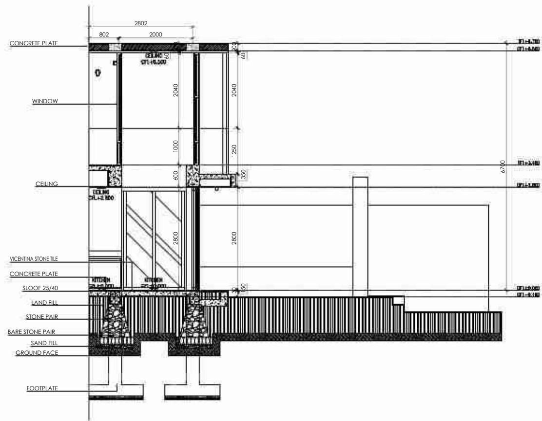
BLOW UP SECTION 1 VILLA C Scale 1 : 100
