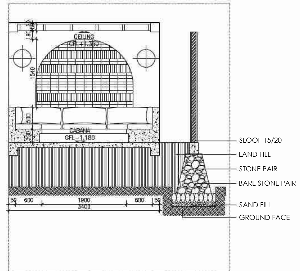
CABANA PLAN, SECTION AND DETAIL VILLA C Scale 1 : 50
