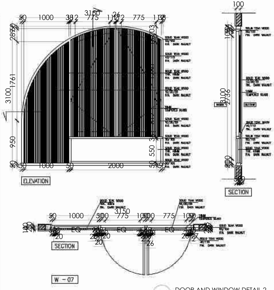
DOOR AND WINDOW DETAIL 2 Scale 1 : 50
