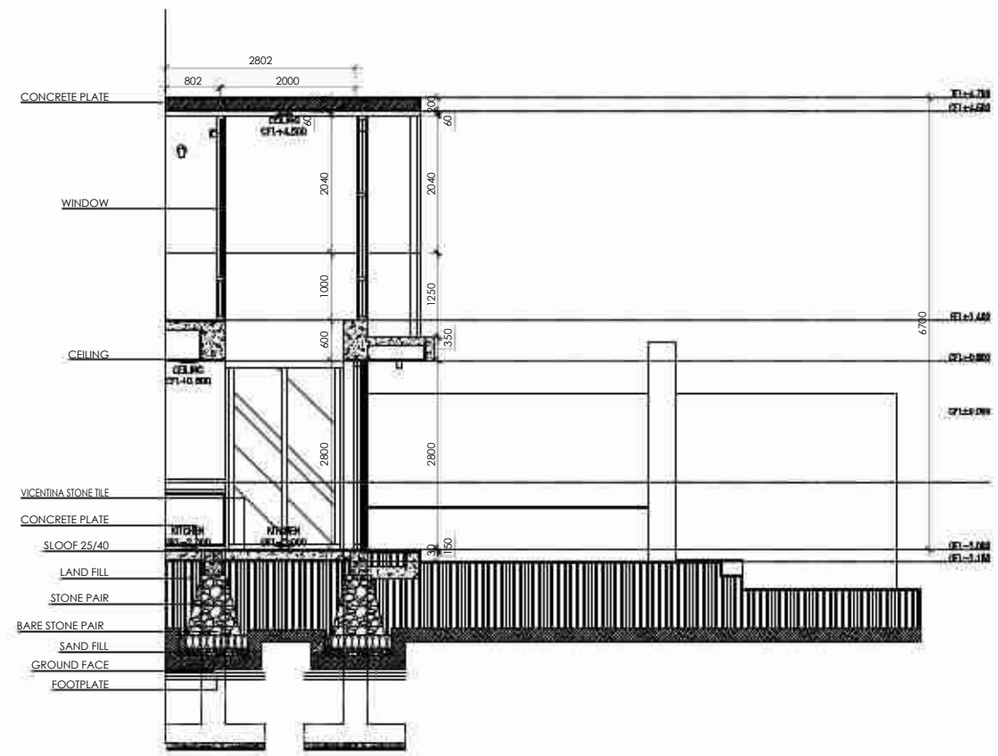
BLOW UP SECTION 1 VILLA A Scale 1 : 100
