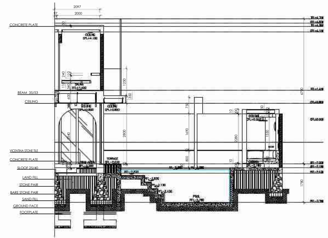
BLOW UP SECTION 2 VILLA A Scale 1 : 100
