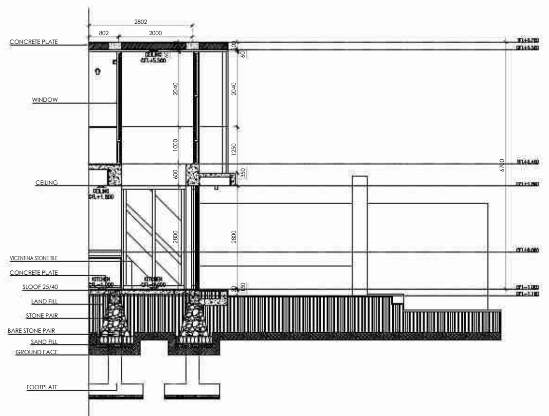
BLOW UP SECTION 1 VILLA B Scale 1 : 100
