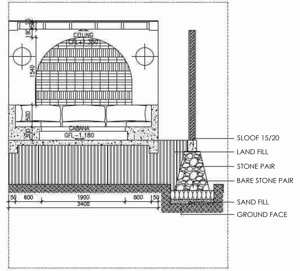
CABANA PLAN, SECTION AND DETAIL VILLA B Scale 1 : 50
